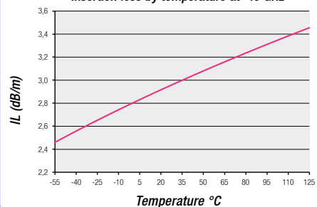
Insertion loss by temperature at 40 GHz
