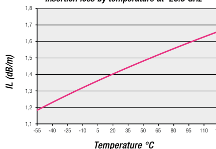
Insertion loss by temperature at 26.5 GHz
