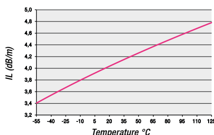
Insertion loss by temperature at 50 GHz
