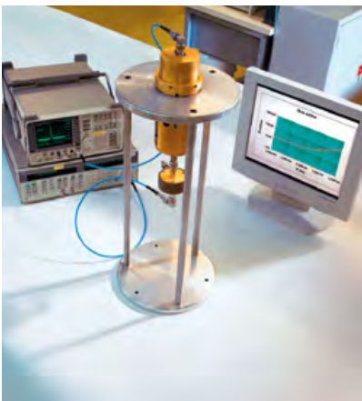
EMI PROTECTION : TRANSFER IMPEDANCE MEASUREMENT
