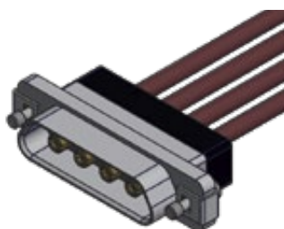
▲ COMBO 51 4 COAX S3 FEMALE PIGTAIL (C1)
