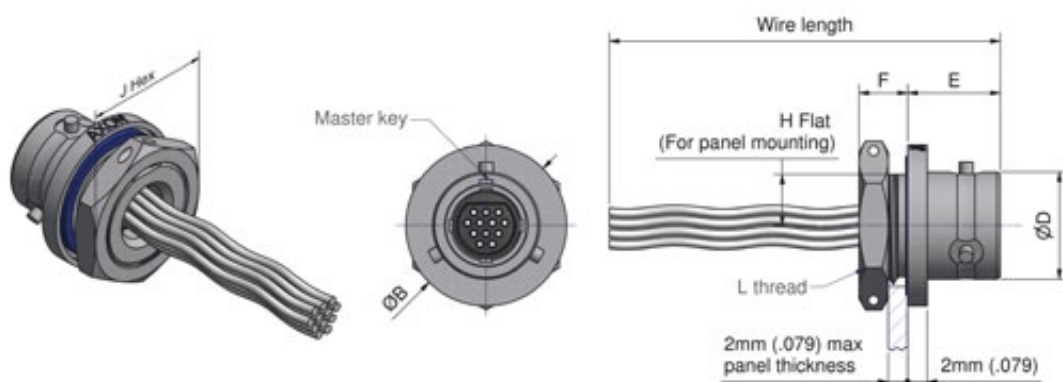
Front mount jam nut female MCA3Bxxx-08Sxxxxxx
