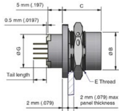
Rear mount jam nut female PCB 0.075" pitch MCABKxxx-12S75Sxxx
