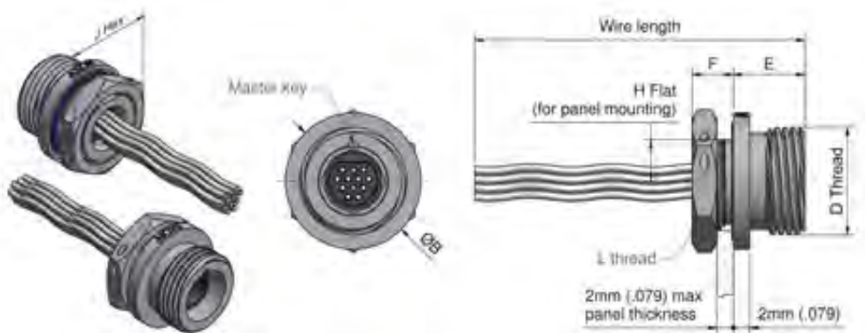
Front mount jam nut female MCACxxx-08Sxxxxxx
