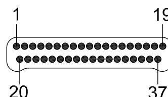
37 CONTACTS
