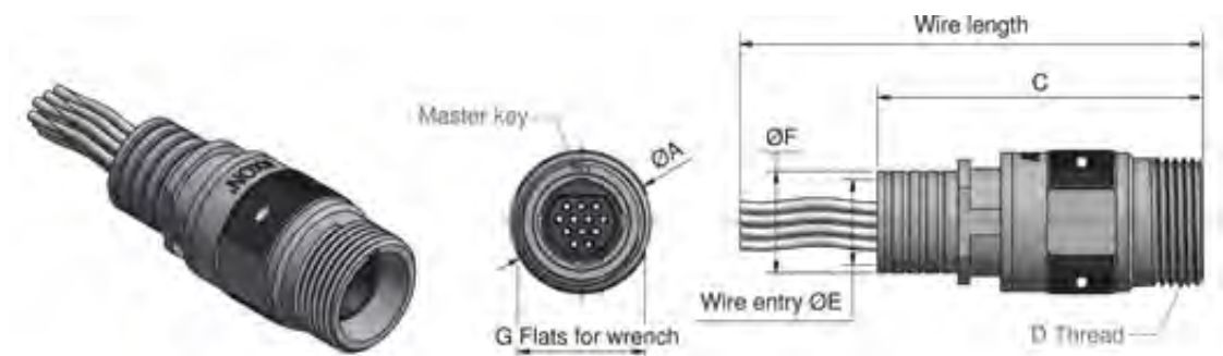
In-line female plug, screen termination funnel
