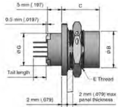
Rear mount jam nut female PCB 0.075" pitch
