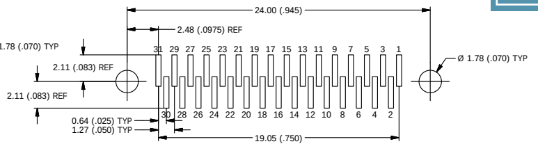
LAYOUT
