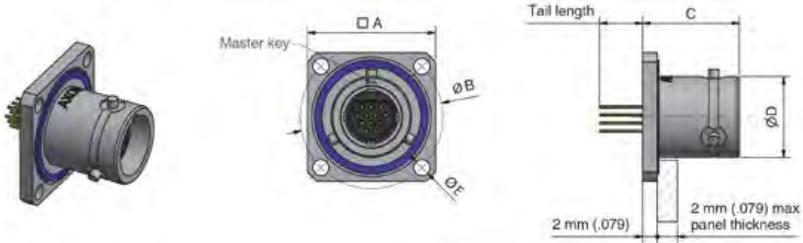
Rear mount square flange female PCB 0.050" pitch MCA3Bxxx-10S50Sxxx
