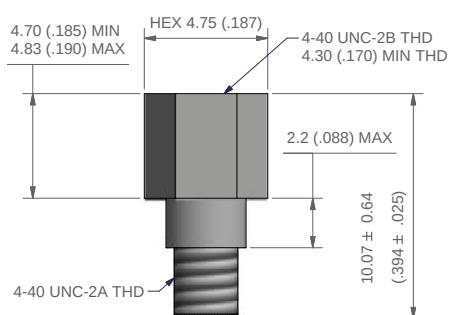
KIT PART NUMBER: MDAHM517SPCB Based on M83513/05-17 Hardware code: P
