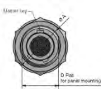
Rear mount jam nut female PCB 0.050" pitch
