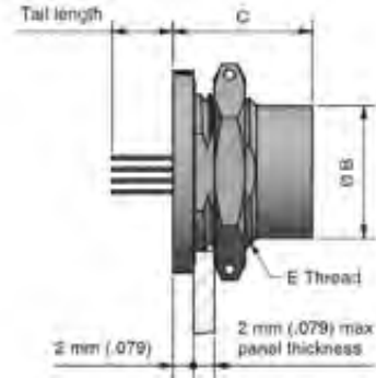
Rear mount jam nut female PCB 0.050" pitch
