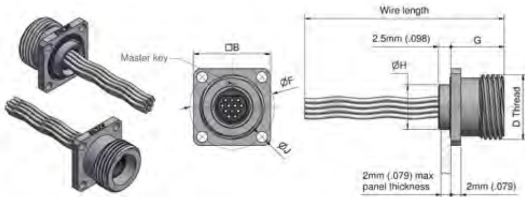
Front mount square flange female
