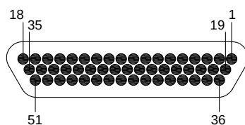
51 CONTACTS
