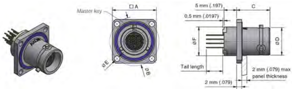
Rear mount square flange female PCB 0.075" pitch MCA3Bxxx-10S75Sxxx
