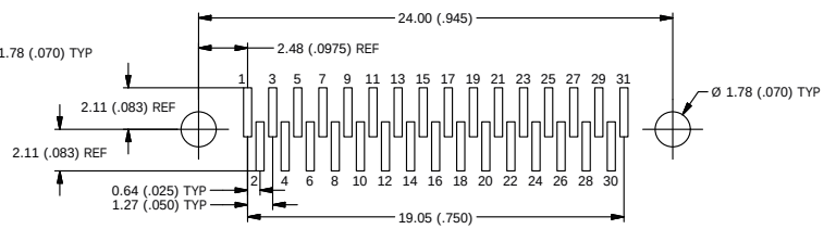
LAYOUT
