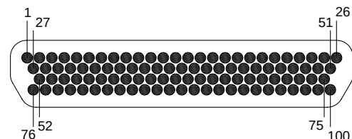
100 CONTACTS
