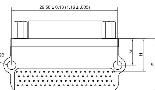
86 way connector
