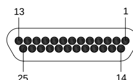
25 CONTACTS
