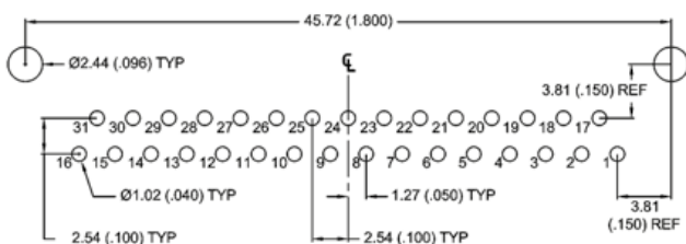
31 CONTACTS - VIEW B
