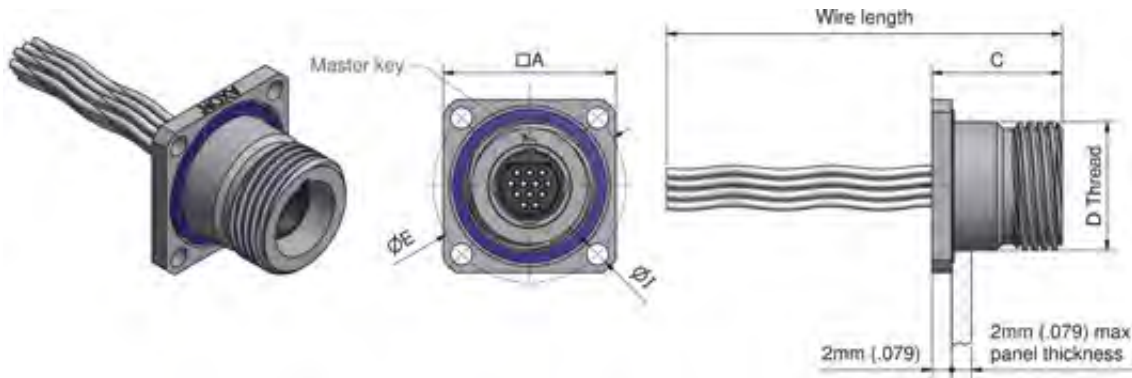
Rear mount square flange female
