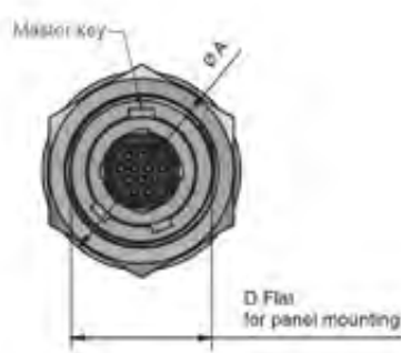
Rear mount jam nut female PCB 0.075" pitch
