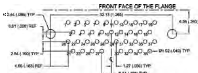
37 CONTACTS - VIEW B
