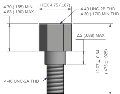
KIT PART NUMBER: MDAHM517SLPCB Based on M83513/05-17 Hardware code: P
