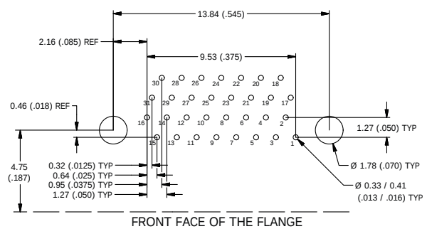
31 CONTACTS - VIEW B
