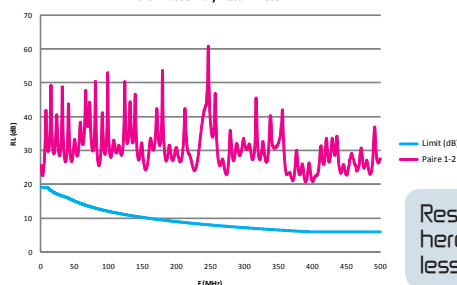
Micro-D assembly Return Loss
