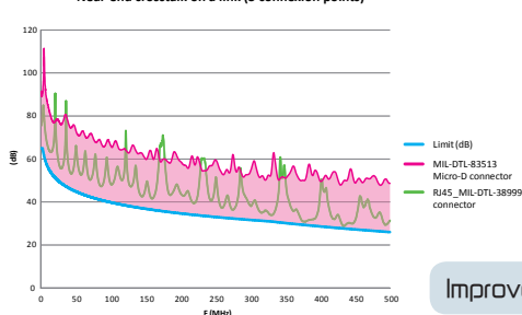
Near-end crosstalk on a link (3 connexion points)
