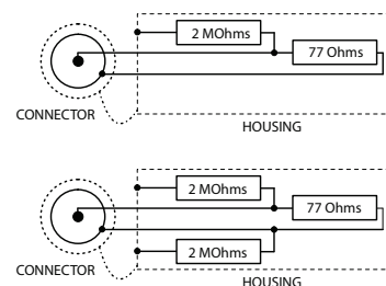
77 \Omega TERMINATOR WITH ESD PROTECTION
